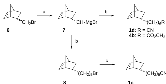
Scheme 3. Synthesis of monomer precursors with long alkyl spacers. a) Mg, THF, 25 °C, 95 %. b) 2 mol % Li_2CuCl_4 , THF, -10 to 25^\circ C , 1d : 6-bromohexanenitrile, 71 % 4b : 6-bromomethylhexanoate, 89 %, 8 : 1,4-dibromobutane, 67 %. c) NaCN, DMSO, 80^\circ C , 3 h, 90 %.
