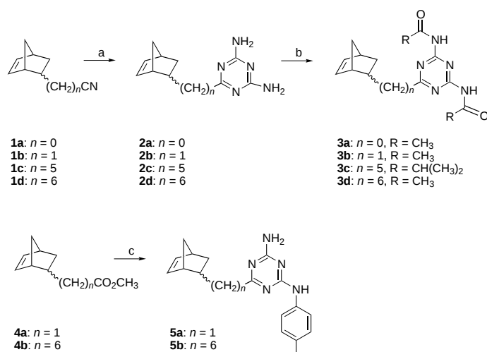
Scheme 2. Synthesis of diaminotriazine monomers 3a–d and 5a–b . a) Dicyanodiamide, KOH, n -propanol, reflux, 12 h, 57–70 %. b) Acetic anhydride, pyridine, 120^\circ C , 1 h, 27–65 % ( 3a, b, d ); isobutyryl chloride, pyridine, 90^\circ C , 2 h, 70 % ( 3c ). c) p -Tolylbiguanide, MeOH, NaOCH 3 , 90^\circ C , 96 h, 41–45 %.
