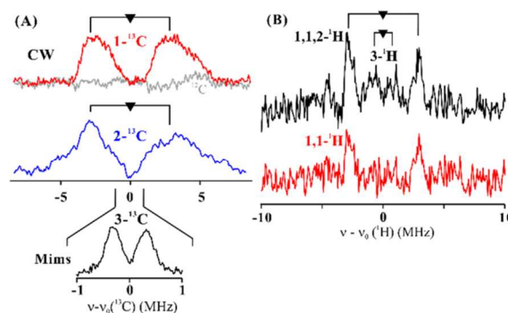
Figure 2. (A) 35 GHz CW 13 C ENDOR spectra for CA with 1- 13 C and 2- 13 C-labeled SAM CA collected at g_2 ; the doublets are split by the hyperfine coupling, and centered at the Larmor
