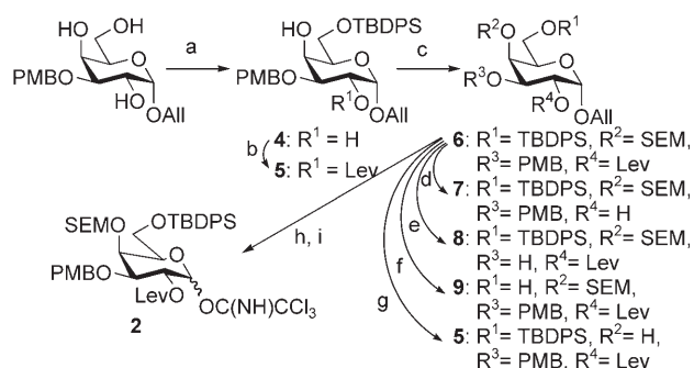
Scheme 2. a) TBDPSCl, CH 2 Cl 2 /Py, 87%; b) Levulinic acid, EDCI, DMAP, CH 2 Cl 2 , 62%; c) SEMCl, DIPEA, CH 2 Cl 2 , 95%; d) NH 2 NH 2 ·AcOH, CH 2 Cl 2 /MeOH, 89%; e) DDQ, CH 2 Cl 2 /H 2 O, 85%; f) TBAF, THF/AcOH, 91%; g) MgBr 2 ·Et 2 O, Et 2 O/CH 3 NO 2 , 87%; h) Ir catalyst, THF, then NBS, THF/H 2 O, 85%; i) Cl 3 CCN, DBU, CH 2 Cl 2 , 85%. DBU = 1,8-diazabicyclo[5.4.0]undec-7-ene, Lev = levulinyl, NBS = N -bromosuccinimide, PMB = p -methoxybenzyl, SEM = [ \beta -(trimethylsilyl)ethoxy]methyl, TBDPS = tert -butyldiphenylsilyl.
