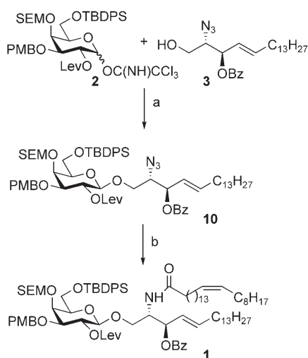
Scheme 1. a) TESOTf, CH 2 Cl 2 , m.s., -50 °C, 86%; b) nervonic acid, Bu 3 P, EDCI, CH 2 Cl 2 , 60%.
