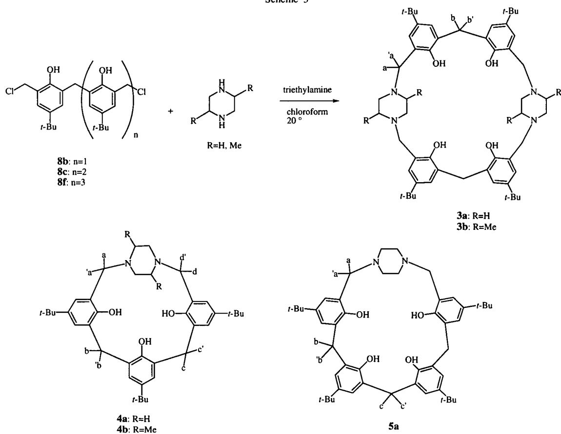
Scheme 3
