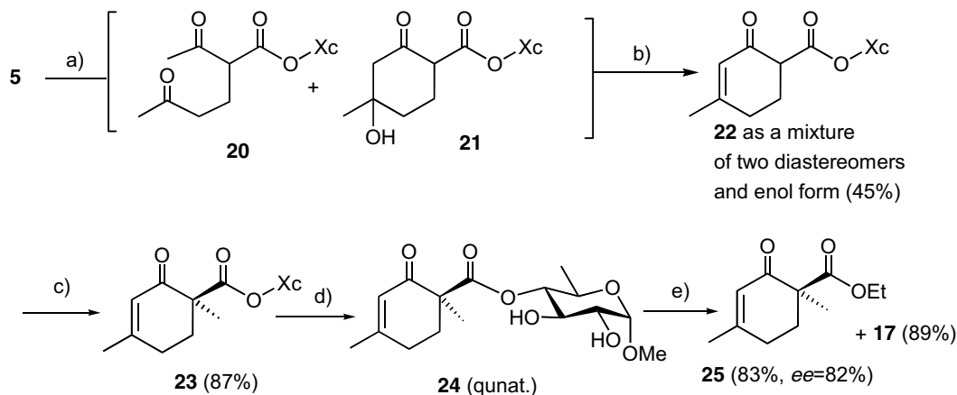
Scheme 4. Synthesis of 25 , the antipode of 16 . Reagents and conditions: (a) methyl vinyl ketone, MeONa/MeOH, -78\text{ }^{\circ}\text{C} (1 h), -18\text{ }^{\circ}\text{C} (1 h), 0\text{ }^{\circ}\text{C} (1 h), rt (24 h); (b) MeONa/MeOH, rt (24 h); (c) MeI, MeONa/MeOH, -78\text{ }^{\circ}\text{C} (0.5 h), -18\text{ }^{\circ}\text{C} (0.5 h), 0\text{ }^{\circ}\text{C} (0.5 h), rt (24 h); (d) 6 M aq HCl/THF (1:1), rt (32 h); (e) EtONa/EtOH, rt (0.5 h).
