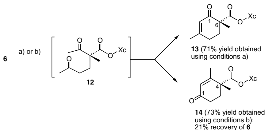
Scheme 2. 1,4-Addition and successive intramolecular cyclization in the reaction of 6 and methyl vinyl ketone. Reagents and conditions: (a) methyl vinyl ketone, MeONa in MeOH, -78 °C (3 h), -18 °C (0.5 h), 0 °C (0.5 h) then rt (3 h); (b) methyl vinyl ketone, pyrrolidine/AcOH, Et 2 O, rt (5 d).
