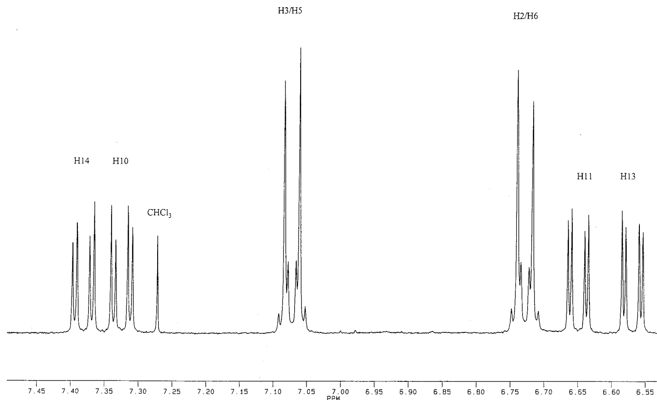
Figure 1. ^1\text{H} NMR spectrum of Diethylnidoaniline ( 6 ) in \text{CDCl}_3 at 50 ^\circ\text{C} .
