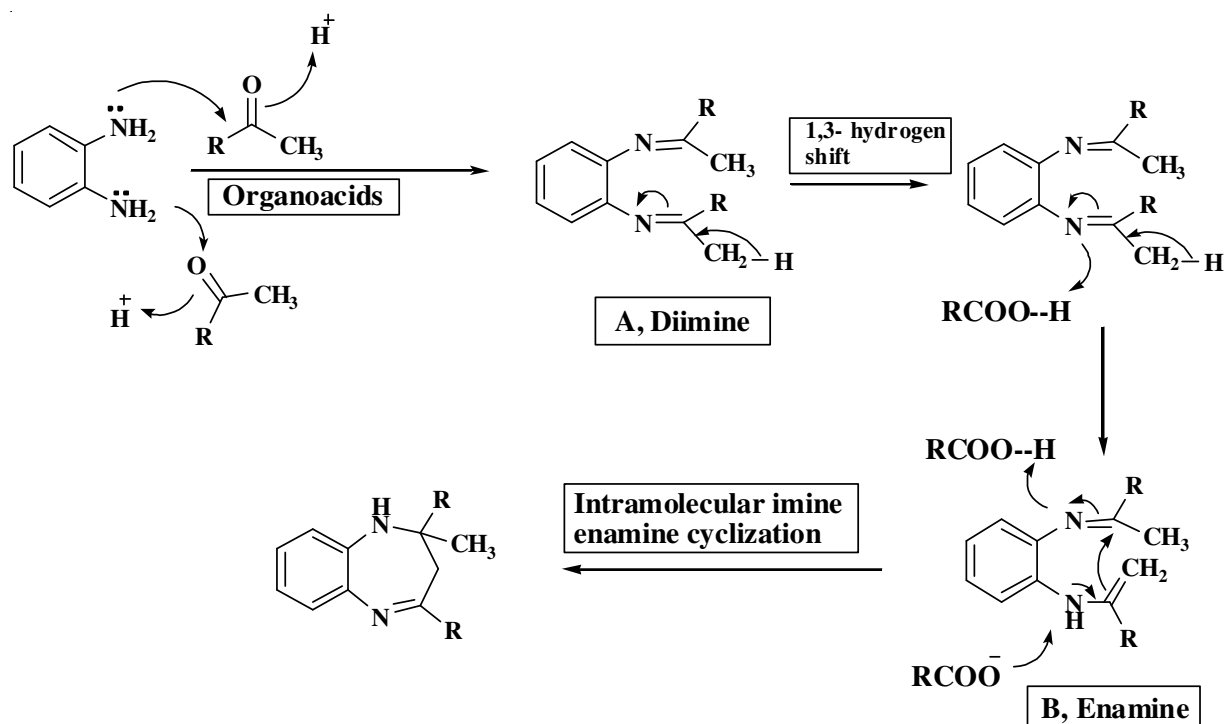
Scheme-II: Proposed mechanism for Bronsted organoacids catalyzed reaction
