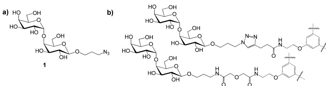
Chart 1 a) Desired galabiose building block for conjugation via “click” chemistry; b) top linkage to dendritic structures compared to previously used linkage (ref. 4 b,d ).
