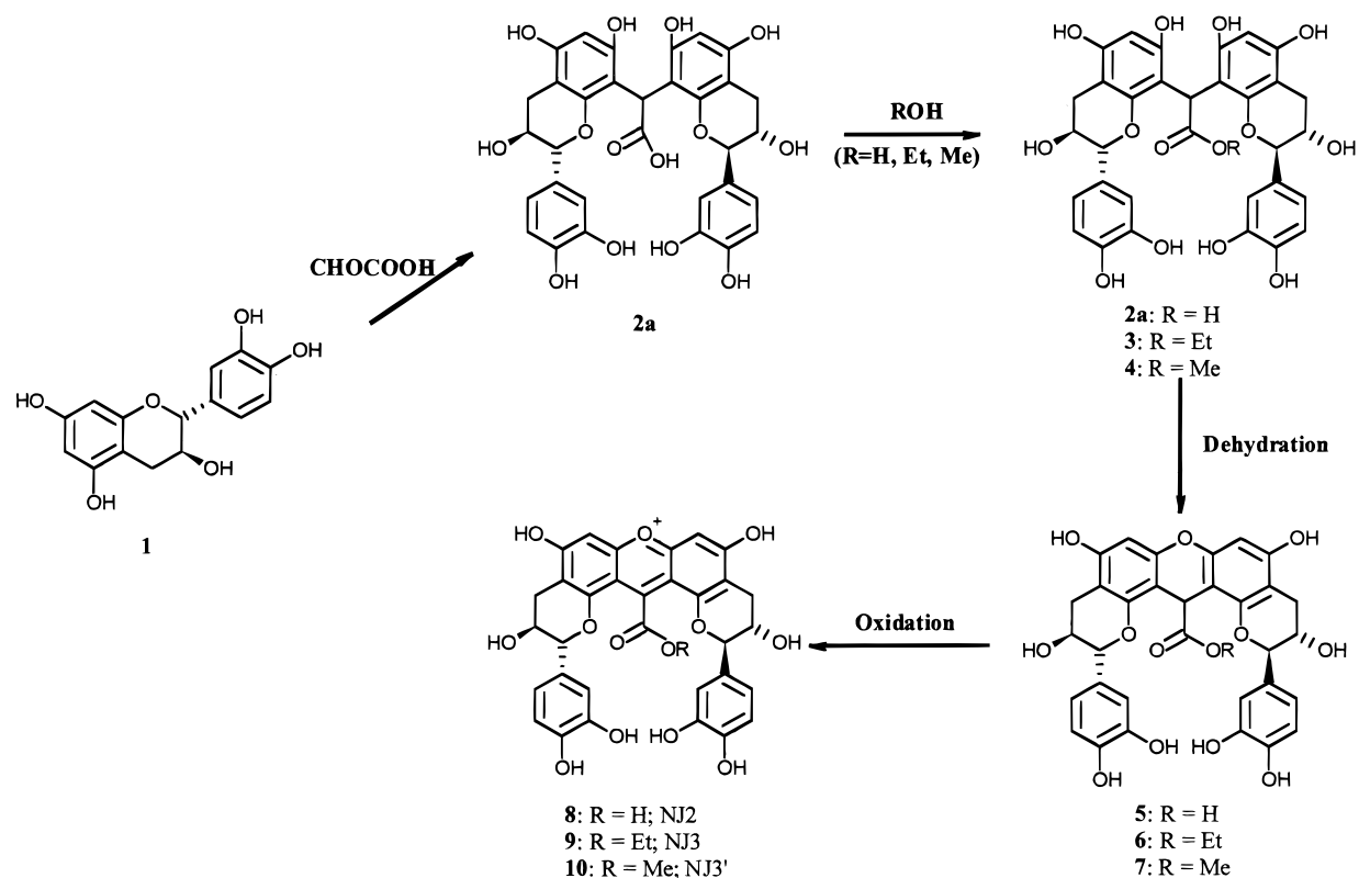
Figure 6. Mechanism of the xanthylium salt 8–10 formation from the colorless dimer 2a via the xanthene derivatives 5–7 .
