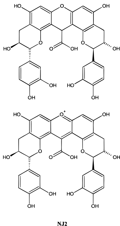
Figure 2. Structures of the xanthene (top) and the xanthylium salt NJ2 (bottom), previously identified (Es-Safi et al., 1999).
