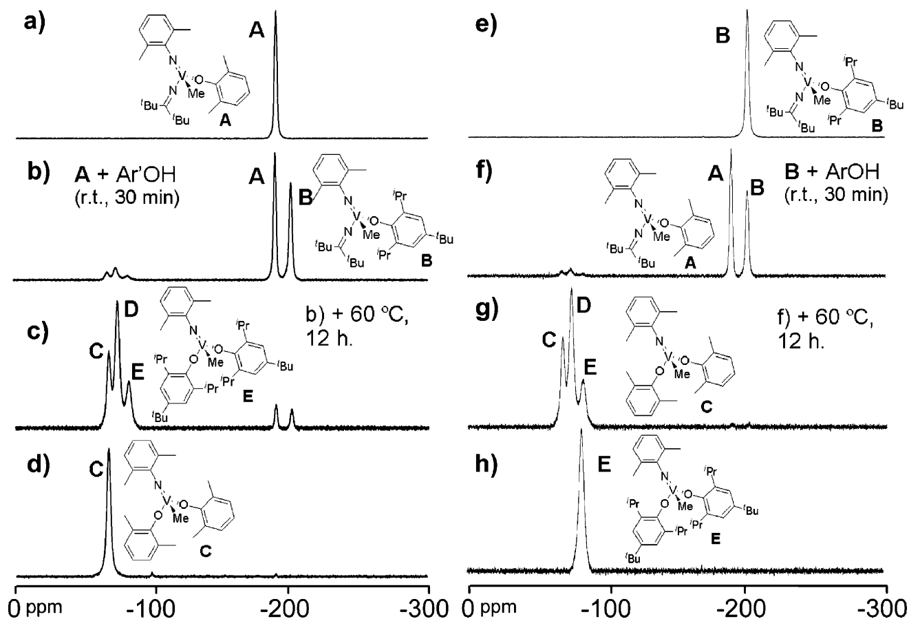
Figure 3. ^{51}\text{V} NMR spectra of the reaction of 2a with 4- t -Bu-2,6- i -Pr 2 C 6 H 2 OH (a–d) and 2b with 2,6-Me 2 C 6 H 3 OH (e–h) in CDCl 3 . ^{51}\text{V} NMR spectra for (a) 2a , (b) reaction mixture of 2a with 4- t -Bu-2,6- i -Pr 2 C 6 H 2 OH (after 30 min at 25 °C), (c) reaction mixture of 2a with 4- t -Bu-2,6- i -Pr 2 C 6 H 2 OH (at 60 °C for additional 12 h after b), and (d) 5a . ^{51}\text{V} NMR spectra for (e) 2b , (f) reaction mixture of 2b with 2,6-Me 2 C 6 H 3 OH (after 30 min at 25 °C), (g) reaction mixture of 2b with 2,6-Me 2 C 6 H 3 OH (at 60 °C for additional 12 h after f), and (h) 5b .
