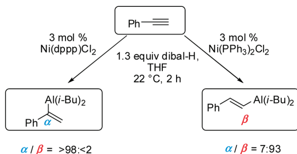
Scheme 2. Selective Generation of \alpha - and \beta -Alkenylalanes 12
