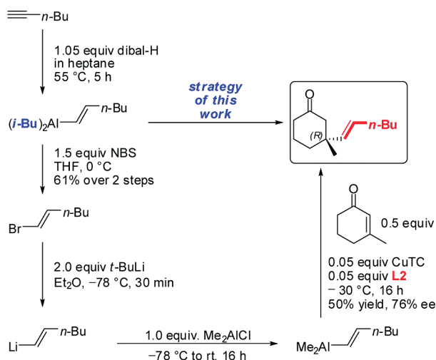
Scheme 1. Direct Use of the ( i Bu) 2 Al-vinyl Nucleophile
