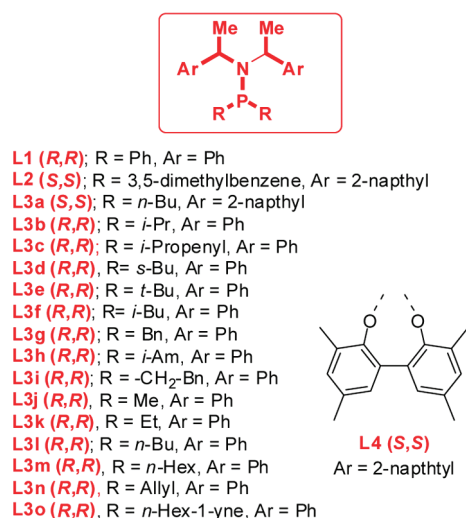
Figure 1. Phosphinamine and phosphoramidite ligand library.
