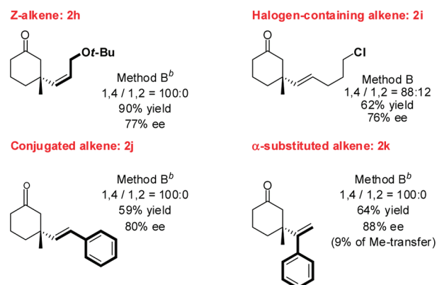
Scheme 3. Further Extension of the Nucleophile Scope a
