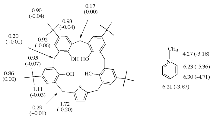
Figure 3. ^1\text{H} Nmr relaxation times T_1 [s] of calixarene analog 1a in the absence of N -methylpyridinium iodide Pyr ^+ at 25^\circ in deuteriochloroform:-deuterioacetonitrile- d_3 = 10:1 (v/v). The figures in the parentheses denote the changes in T_1 in the presence of Pyr ^+ .
