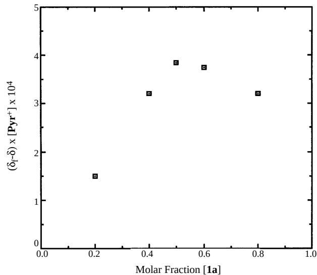
Figure 4. Job's plot. (δ I -δ) is shift in ppm induced in the NCH 3 proton of Pyr + , and the total concentration of 1a plus Pyr + maintained at 10 mM in deuteriochloroform:deuteroacetonitrile-d 3 = 10:1 (v/v) at 20°.
