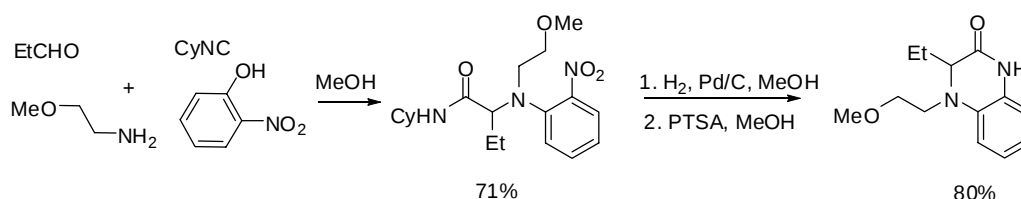
Scheme 2: dehydroquinoxalinone formation
