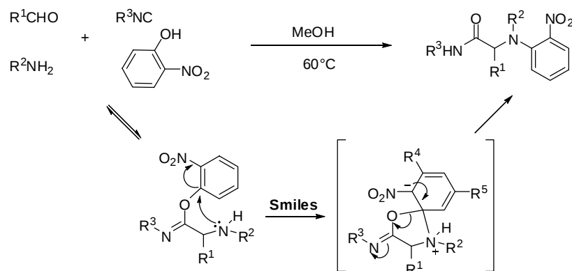
Scheme 1: Ugi/Smiles coupling
