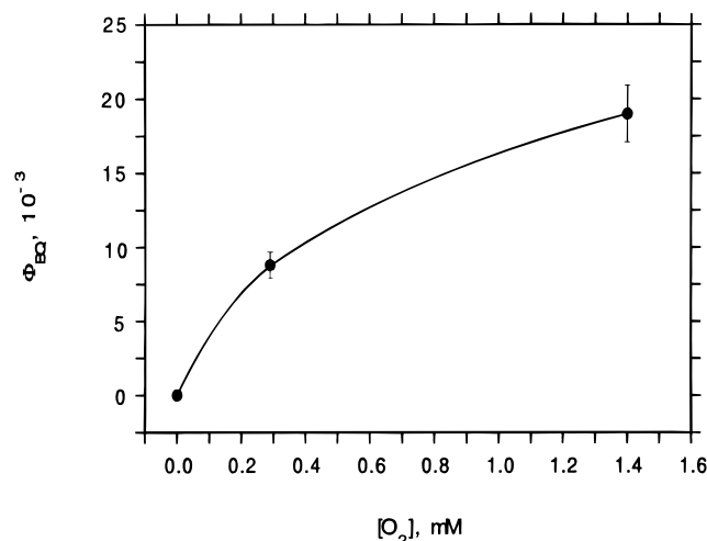
Figure 1. \Phi_{\text{BQ}} as a function of [\text{O}_2] for aqueous solutions of 40 \mu\text{M} \text{Ru}(\text{bpy})_3^{2+} and 4.0 \text{ mM} \text{PhOH} at 20^\circ\text{C} and \text{pH } 6.0 . Error bars are \pm 10\% . The solid curve is a fit of eq 6.
