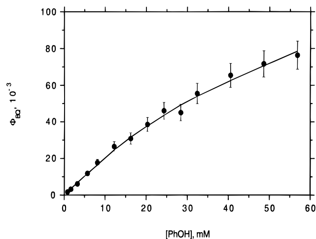
Figure 2. \Phi_{\text{BQ}} as a function of [\text{PhOH}] for air-saturated aqueous solutions of 40 \mu\text{M} \text{Ru}(\text{bpy})_3^{2+} at 20^\circ\text{C} and \text{pH } 6.0 . Error bars are \pm 10\% . The solid curve is a fit of eq 6.
