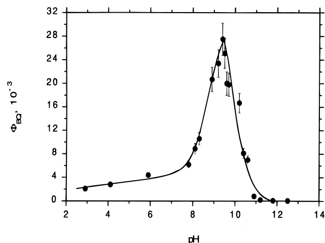
Figure 3. \Phi_{\text{BQ}} as a function of \text{pH} for air-saturated aqueous solutions of 80 \mu\text{M} \text{Ru}(\text{bpy})_3^{2+} and 2.0 \text{ mM} \text{PhOH} at 20^\circ\text{C} . Error bars are \pm 10\% . The solid curve is a fit of eq 16.
