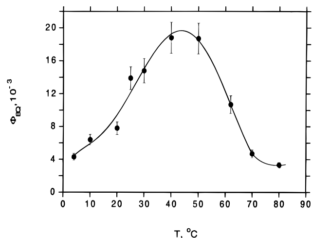
Figure 4. \Phi_{\text{BQ}} as a function of temperature for air-saturated aqueous solutions of 80 \mu\text{M} \text{Ru}(\text{bpy})_3^{2+} and 3.2 \text{ mM} \text{PhOH} at \text{pH } 6.0 . Error bars are \pm 10\% .
