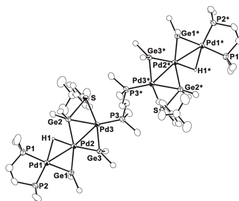
Figure 2. Thermal ellipsoids (30%) of 3 . The molecule has a crystallographic point of symmetry at the midpoint of P3 and P3*. Selected bond distances (Å) and angles (deg): Pd1–Pd2 2.799(2), Pd2–Pd3 2.767(2), Pd3–S 2.501(3), Pd1–Ge1 2.436(2), Pd2–Ge1 2.386(2), Pd2–Ge2 2.411(2), Pd2–Ge3 2.380(2), Pd3–Ge2 2.582(2), Pd3–Ge3 2.407(2), Ge2–S 2.466(3), Pd1–H1 2.2(1), Pd2–H1 2.0(2), Pd1–Pd2–Pd3 168.54(4), Pd2–Pd3–S 110.71(7), Pd1–Ge1–Pd2 70.94(5), Pd2–Ge2–Pd3 67.20(5), Pd2–Ge3–Pd3 70.63(5).
