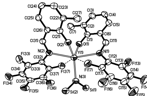
Fig. 3. Molecular structure of Y\{N(SiMe_3)_2\}(L^3)_2 ( 7 ), showing the atomic numbering scheme. Ellipsoids are drawn at 50% probability.
