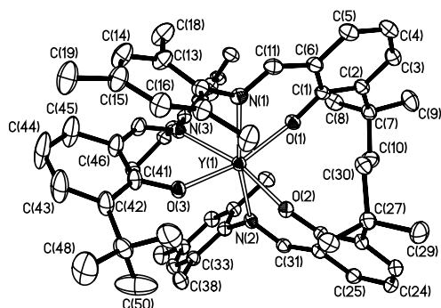
Fig. 2. Molecular structure of Y(L^1)_3 ( 3 ), showing the atomic numbering scheme. Ellipsoids are drawn at 50% probability.
