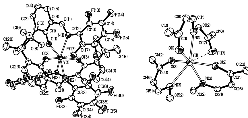
Fig. 4. Molecular structure of Y(L 1 ) 3 ( 8 ). Left: structure showing the atomic numbering scheme. Right: coordination geometry of 8 , with most ligand atoms omitted for clarity.
