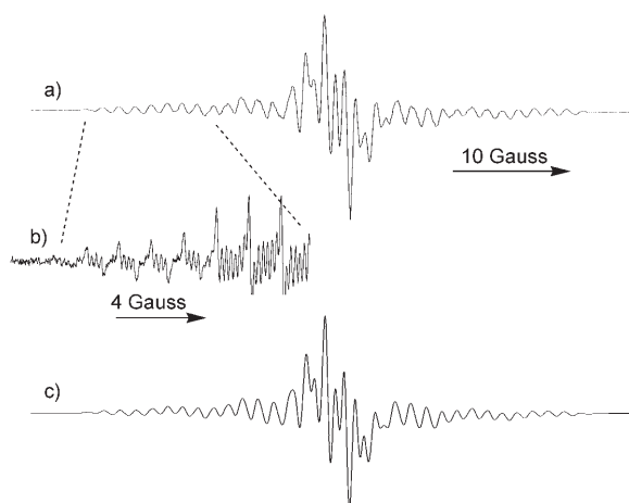
Figure 2. a) Experimental EPR spectrum obtained by photolysis of a mixture of 4 ( 7.5 \times 10^{-3} M) and BHA ( 2.1 \times 10^{-4} M) in degassed benzene containing 10% di-tert -butyl peroxide at room temperature and c) the computer simulated spectrum. b) The expansion of the first part of the of the high-resolution EPR spectrum of the phenoxyl radical from 4 .
