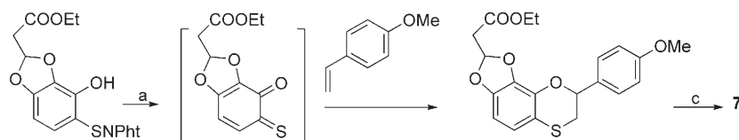
Scheme 2. Reagents and conditions: a) Et 3 N, CHCl 3 , 60–70 °C; b) TBAF·3H 2 O, THF, 0 °C; c) pyrrolidine, CH 3 CN, RT. PG = protecting group, TBAF = tetra- n -butylammonium fluoride.
