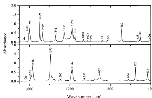
Figure 4. IR spectra of phenol (A) and hexadeuteriophenol (B) in the 1700–400 cm -1 region in CCl 4 solution.
