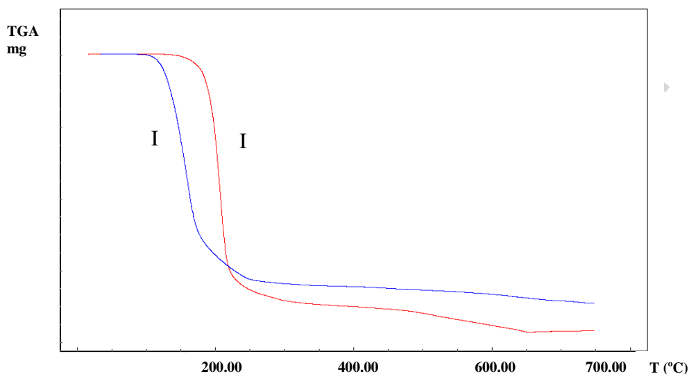
Figure 2. TGs curves for compounds I (red) and II (blue).
