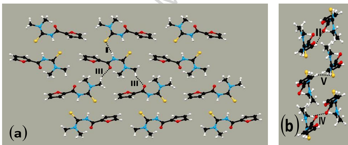
Figure 7. (a) Layer view along a normal to [1,0,2]. (b) Two layers view along b axis direction in the compound II .
