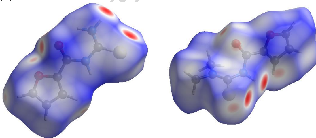
(B) Full fingerprint plot
