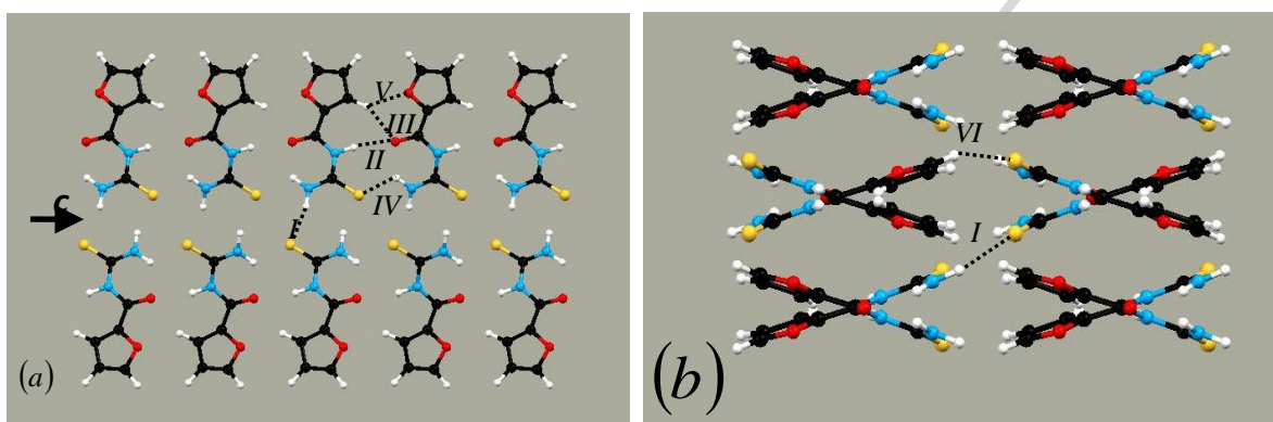
Figure 6. (a) Two chains view along b axis direction, in the compound I . (b) Six chains view along c axis direction.
