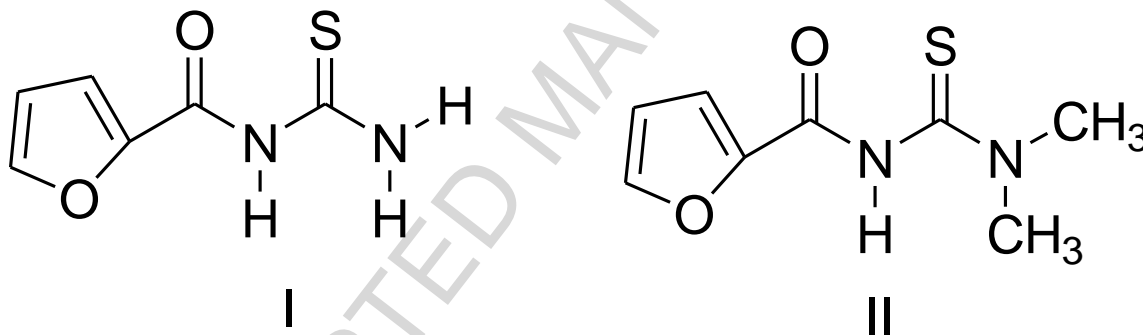
Scheme 2. 1-(2-furoyl) thioureas I and II studied in this work.
