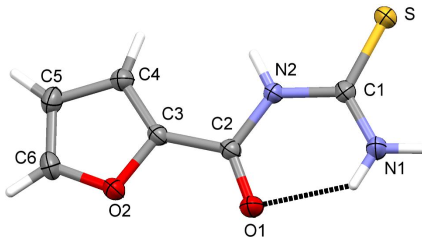
Figure 4. The molecule structure of the compound I in the crystal. Ellipsoids represent 50% probability levels and dashed line indicates intramolecular hydrogen bond.
