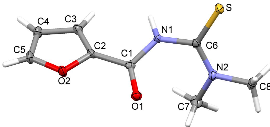
Figure 5. Molecular structure of compound II . Displacement ellipsoids are drawn at the 50% probability level.
