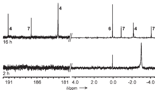
Figure 7. 13 C{ 1 H} NMR spectra of 8 after 2 h (bottom) and after 16 h (top) at ambient temperature.
