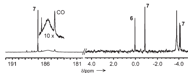
Figure 5. In situ 13 C{ 1 H} NMR spectrum of the reduction of 13 CO 2 with 2 in the presence of a catalytic amount of 3 after complete consumption of 2 (79 h).
