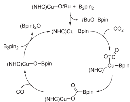
Scheme 1. Simplified Mechanism of the Copper-Catalyzed Reduction of CO 2 to CO with B 2 pin 2 According to DFT Calculations 5
