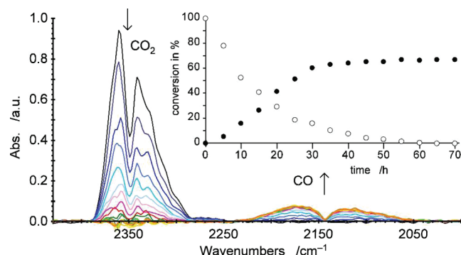
Figure 4. Detail of time-dependent IR spectra during the reduction of CO 2 to CO with 2 in the presence of catalytic amounts of 3 . Inset: Conversion of CO 2 to CO (○, amount of CO 2 ; ●, amount of CO). 8
