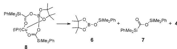
Figure 6. Molecular structure of 8 ; the aromatic rings are represented by the ipso -carbon atom only (spheres). Selected bond lengths [Å] and angles [°]: Cu1–C1 1.869(7), Cu1–O1 1.988(4), Cu1–O3 2.248(4), Cu1–O5 2.315(5), C1–Cu1–O1 151.3(3), C1–Cu1–O3 116.3(2), C1–Cu1–O5 119.0(3). 8
