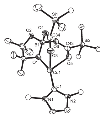
Figure 6. Molecular structure of 8 ; the aromatic rings are represented by the ipso -carbon atom only (spheres). Selected bond lengths [Å] and angles [°]: Cu1–C1 1.869(7), Cu1–O1 1.988(4), Cu1–O3 2.248(4), Cu1–O5 2.315(5), C1–Cu1–O1 151.3(3), C1–Cu1–O3 116.3(2), C1–Cu1–O5 119.0(3). 8
