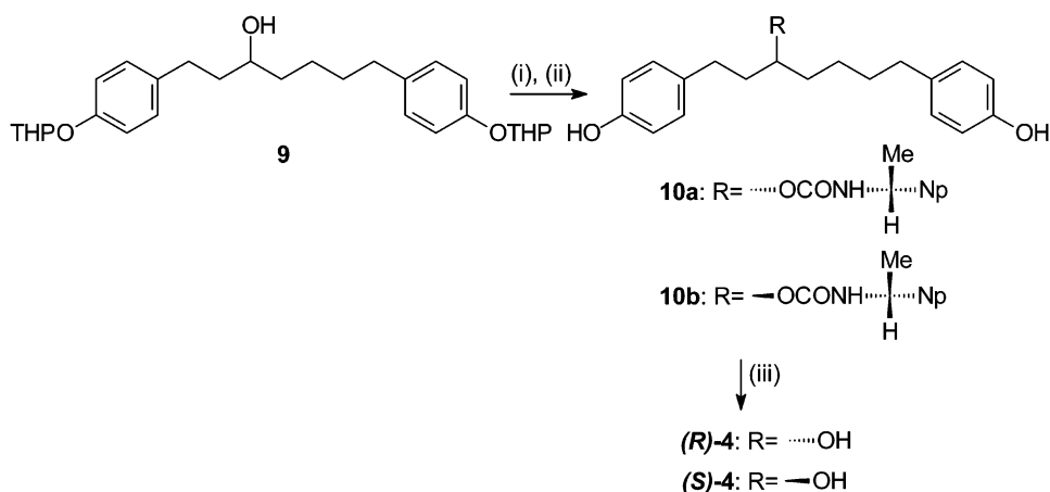
Figure 4. Resolution of centrololol: (i) BF 3 ·etherate; (ii) ( R )-1-(1'-naphthyl)ethyl isocyanate; (iii) LiAlH 4 , Et 2 O.
