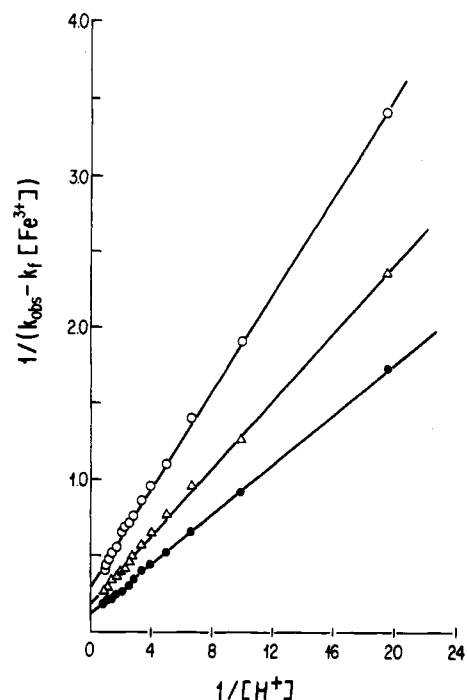
Figure 1. 1/(k_{\text{obsd}} - k_f[\text{Fe}^{3+}]) vs. 1/[\text{H}^+] plot for the acid-catalyzed aquation of \text{FeSal}^+ . Correlation coefficient is 0.999 at 20 °C (open circles), 25 °C (triangles), and 30 °C (closed circles).
