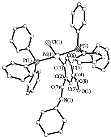
Fig. 1. Molecular structure of [\text{Pd}\{4-(\text{CHO})\text{C}_6\text{H}_3\text{C}(\text{H})=\text{NCy}\}(\text{Cl})(\text{PPh}_3)_2] ( 2 ), with labeling scheme. Hydrogen atoms have been omitted for clarity.
