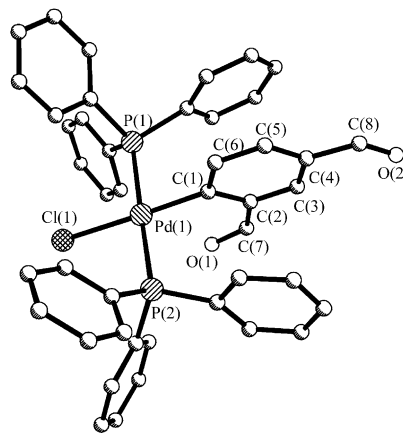
Fig. 2. Molecular structure of [\text{Pd}\{2,4-(\text{CHO})_2\text{C}_6\text{H}_3\}(\text{Cl})(\text{PPh}_3)_2] ( 6 ), with labeling scheme. Hydrogen atoms have been omitted for clarity.
