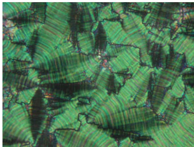
Fig. 2 Texture of the B H phase (identified with the B 2 phase) observed at T = 187\text{ °C} under crossed polarizers with horizontal and vertical polarization directions. The width of the picture is 400 \mu\text{m} .
