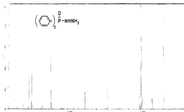
Figure 1. Mass spectrum of diphenylphosphinohydrazide (Ia).
