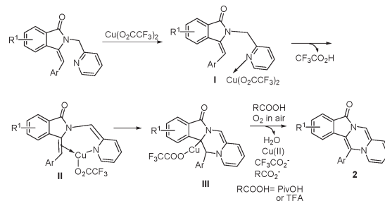
Scheme 1. Possible Mechanism for Copper-Catalyzed Aerobic Oxidative Intramolecular Alkene C–H Amination Leading to N -Heterocycles ( 2 )
