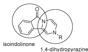
Figure 1. Structure of conjugate containing isoindolinone and 1,4-dihydropyrazine frameworks.
