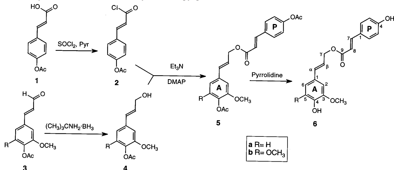
Scheme 1. Synthetic Scheme for Coniferyl and Sinapyl p -Coumarates
