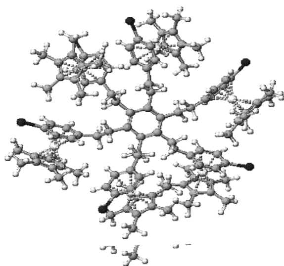
Figure 1. Molecular modeling calculations for 4 were carried out using CAChe. The optimized geometry was calculated with MM2 using augmented MM3 parameters to an average gradient less than 1. The conformation with minimized energy was obtained from the optimized molecule using the sequential search option in the software package. The Ru–Cp* distances were found to be the same as in known crystal structures containing this fragment. 7
