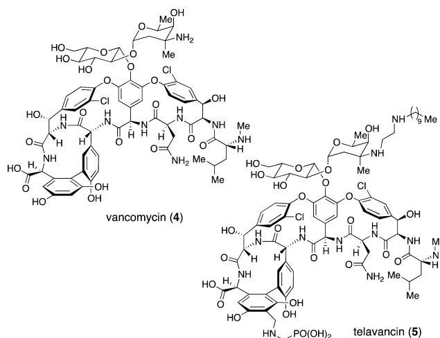
Figure 2. Structure of the representative glycopeptide drugs vancomycin (4) and telavancin (5).
