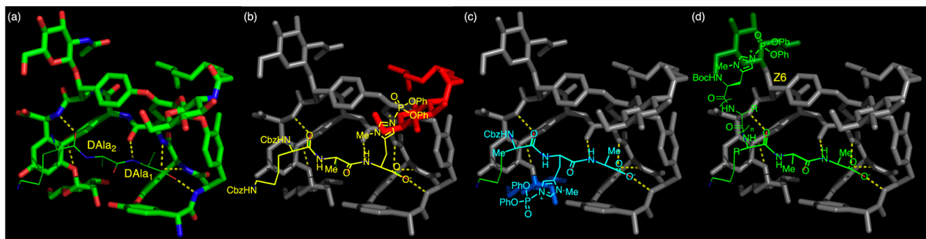
Figure 3. Design of peptide catalysts based on the X-ray crystal structure of DAla–DAla containing peptide bound to teicoplanin: (a) X-ray crystal structure of Lys–DAla–DAla–O − ( 6 , lines) bound to 6c-dechloroteicoplanin ( 7 , sticks, adapted from PDB 3VFG). 46 (b) Proposed model for delivery of the diphenylphosphoryl group to the N -decanoylglucosamine ring by Z-Lys(Z)–DAla–DPmh–O − . (c) Proposed model for delivery of the diphenylphosphoryl group to the mannose ring by Z-Ala–DPmh–DAla–O − . (d) Proposed model for delivery of the diphenylphosphoryl group to the N -acetylglucosamine ring by Pmh-(Xaa) n –DAla–DAla–O − .
