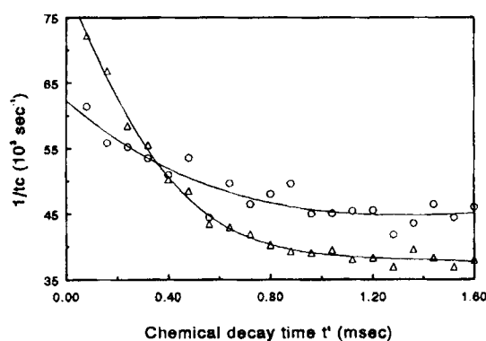
Figure 3. Typical inverse photon decay time plot obtained by the photolysis of C 6 H 5 OCH 3 -NO-Ar mixture at 193 nm. The measurements were carried out at (Δ) 297 K with [NO] = 1.11 \times 10^{15} molecules cm -3 and (○) 373 K with [NO] = 9.31 \times 10^{14} molecules cm -3 , respectively. The solid curves are the least-squares fit to equation (9)
