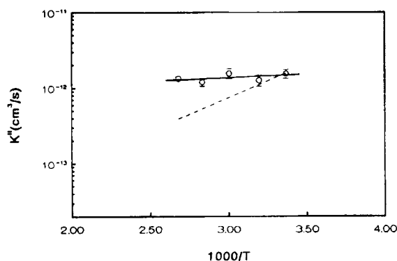
Figure 5. Arrhenius plots of the bimolecular rate constants for \text{C}_6\text{H}_5 + \text{NO} \rightarrow (\text{C}_6\text{H}_5\text{O})\text{NO} from the experiment (40 Torr). The dashed line represents the results evaluated by equation (1). The solid line is the least-squares fit to the results obtained by equation (5), which takes into account the effect of the reverse reaction
