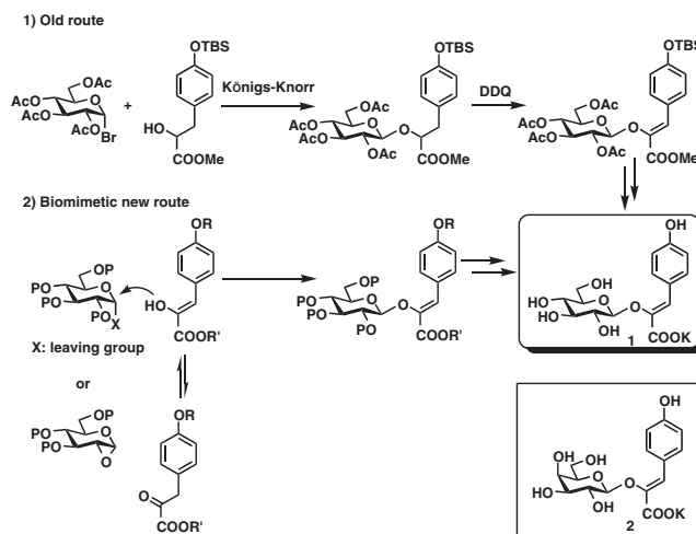
Figure 1. Old synthetic route and Biomimetic new route to 1 .
