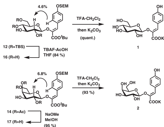
Scheme 1. Synthesis of 1 and 2 .
