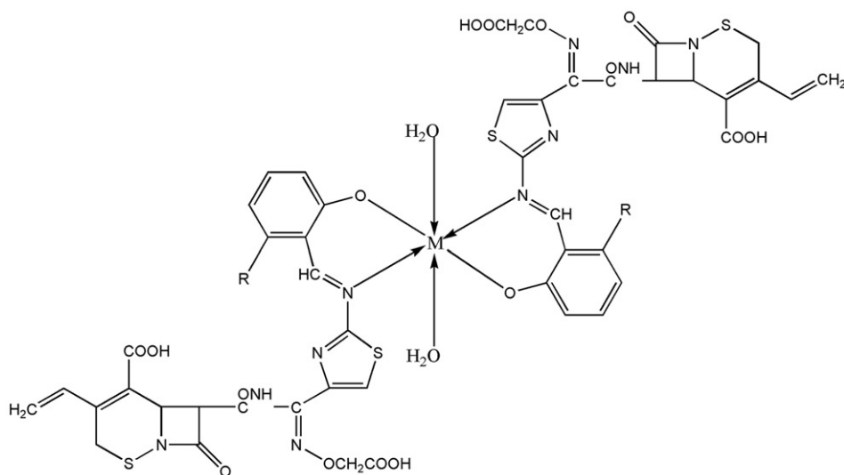
Figure 2. Proposed structure of metal complexes of L_1 and L_2 , where R = H and phenyl; M = Zn(II) , Cu(II) , Ni(II) , and Co(II) .
