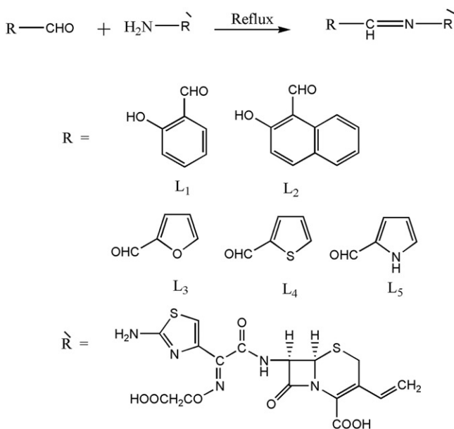
Figure 1. Proposed structure of Schiff-base ligands.
