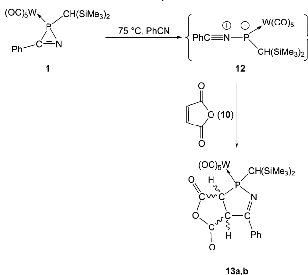
Scheme 5. \pi -Selective Reaction of Transient Nitrilium Phosphane-ylide Complex 12 with Alkene 10 under Formation of Bicyclic 1,2-Azaphosphol-5-ene Complexes 13a,b
