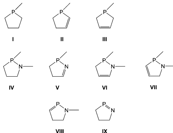
Scheme 1. λ 3 -Phospholanes ( I–III ), 1,2λ 3 -Azaphospholanes ( IV ), and 1,2λ 3 -Azaphospholenes ( V–IX ) (lines denote ubiquitous organic substituents)
