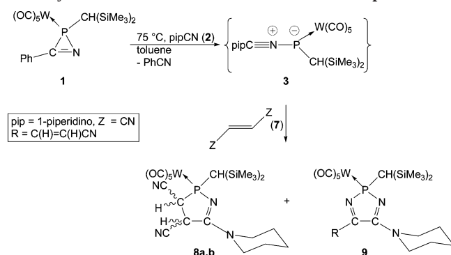
Scheme 4. Formation of C 5 -Spirocyclic 1,3,2-Oxazaphosphol-3-ene Complexes 11a,b
