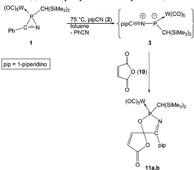
Scheme 4. Formation of C 5 -Spirocyclic 1,3,2-Oxazaphosphol-3-ene Complexes 11a,b
