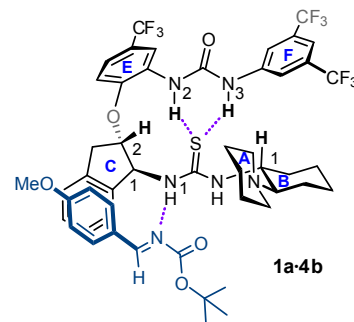
Figure 6. Summary of 1 H NMR shifts observed when catalyst 1a was titrated with a) acetylacetonate ( acac ) or b) imine 4b .
