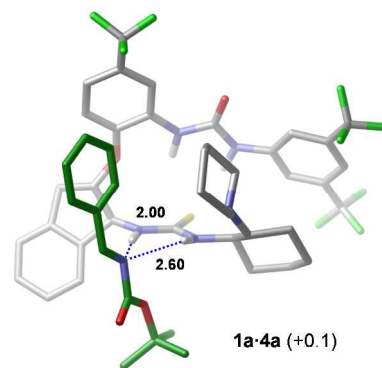
Figure 5. The most stable form of complex 1a·4a and the ion pair formed upon substrate deprotonation. Relative stability (in kcal/mol; with respect to 1a + 4a ) is given in parenthesis.
