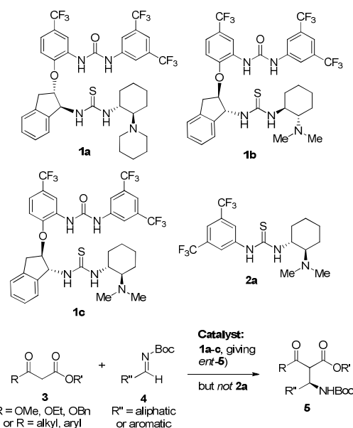
Scheme 1. Catalysts 1a-1c and 2a and their contrasting reactivity
