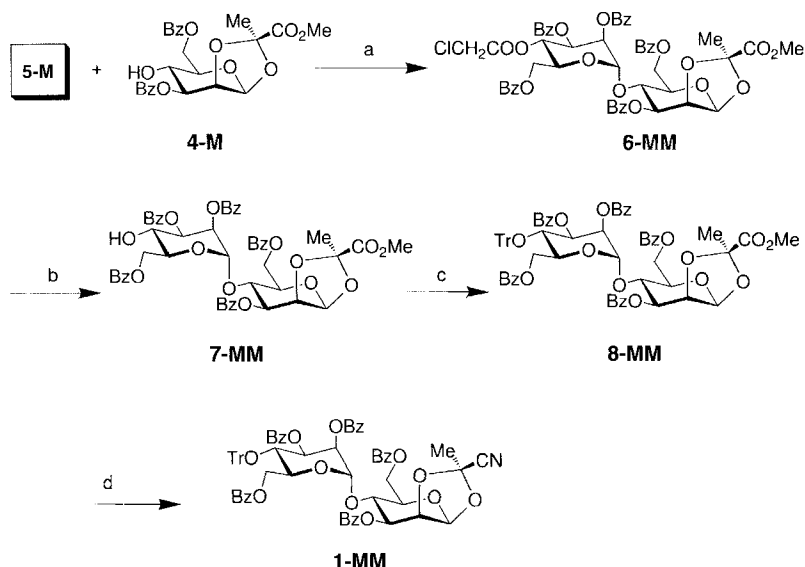
Scheme 8. Synthesis of the L-mannosyl-D-mannose disaccharide monomer 1-MM from the glycosyl donor 5-M and the glycosyl acceptor 4-M . Reagents and conditions: a) \text{AgOTf/collidine}/\text{CH}_2\text{Cl}_2 , -30^\circ\text{C} , 1 h, 67%; b) (\text{H}_2\text{N})_2\text{CS}/\text{MeCN}/\text{H}_2\text{O} , 48 h, 20^\circ\text{C} , 87%; c) \text{TrClO}_4/\text{collidine}/\text{CH}_2\text{Cl}_2 , 20^\circ\text{C} , 4 h, 84%; d) i) \text{NH}_3/\text{MeOH}/\text{CH}_2\text{Cl}_2 , -5 to 20^\circ\text{C} , 18 h, ii) \text{BzCl}/\text{C}_6\text{H}_5\text{N} , 20^\circ\text{C} , 18 h, 74%.
