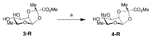
Scheme 2. Synthesis of the L-rhamnose glycosyl acceptor 4-R . Reagents and conditions: a) \text{BzCN}/\text{C}_2\text{H}_5\text{N}/\text{CH}_2\text{Cl}_2 , 20^\circ\text{C} , 18 h, 58%.
