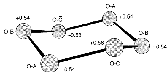
Figure 17. The polygon formed by the six glycosidic oxygen atoms of the cyclic hexasaccharide 29 . The distances (Å) from the mean plane of this ring are shown beside each oxygen atom. The speckled grey balls represent the six glycosidic oxygen atoms.
