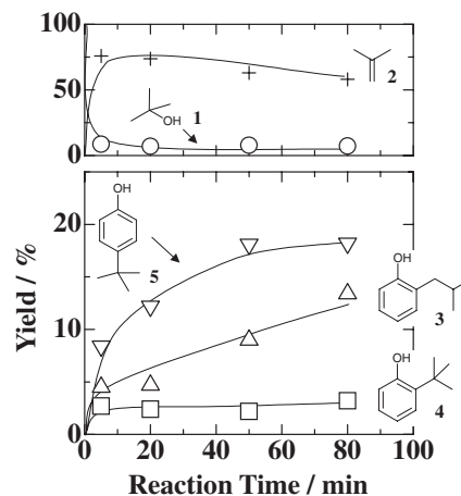
Figure 1. Yield of (+) isobutene (2), ( \Delta ) 2-isobutylphenol (3), ( \square ) 2- tert -butylphenol (4), ( \nabla ) 4- tert -butylphenol (5) for reaction of phenol with tert -butyl alcohol (○) at 0.5 g/cm 3 of water density and 673 K.
