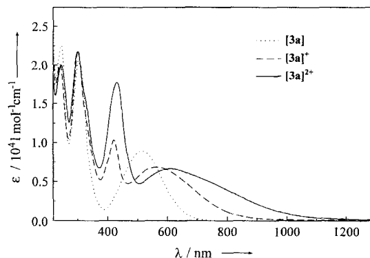
Figure 13. Electronic spectra of 3a , [3a]\text{ClO}_4 and electrochemically generated [3a]^{2+} in CH 3 CN.
