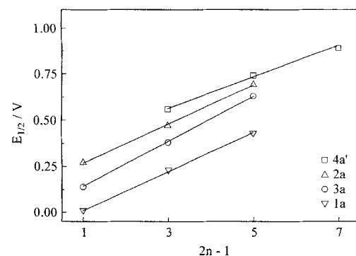
Figure 10. Dependence of the redox potentials E_{1/2}^1 , E_{1/2}^2 , E_{1/2}^3 of the couples [\text{LM}]^{n+}/[\text{LM}]^{(n+1)+} on 2n-1 where n represents the charge of the species [\text{LM}]^n . The solid lines are for guidance only.
