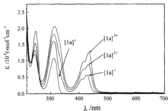
Figure 12. Electronic spectra of 1a and electrochemically generated [1a]^{+} , [1a]^{2+} and [1a]^{3+} in CH 3 CN (0.10 M [N(n\text{Bu})_4]\text{PF}_6 ).
