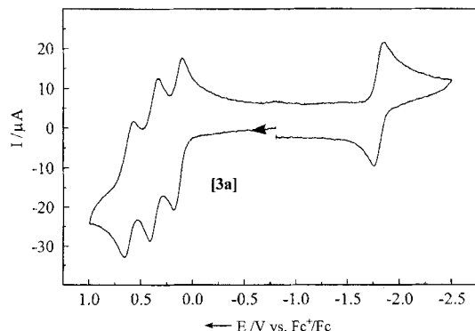
Figure 8. Cyclic voltammogram of 3a in \text{CH}_3\text{CN} (conditions as given in Figure 6).
