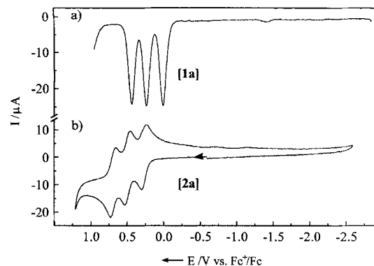
Figure 7. Cyclic voltammogram of 2a in \text{CH}_3\text{CN} (conditions as given in Figure 6) and square-wave voltammogram of 1a in \text{CH}_3\text{CN} (0.10 M [\text{N}(\text{nBu})_4]\text{PF}_6 ; frequency: 30 Hz; pulse height 2.5 \times 10^{-2} V; glassy carbon electrode).
