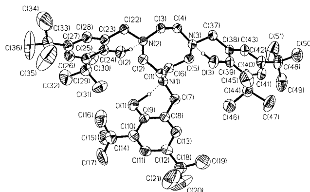
Figure 1. Structure of the ligand L^{Bu}H_3 . Intramolecular O \cdots H \cdots N contacts [ \text{\AA} ]: O(1) \cdots N(1) 2.623(5), O(2) \cdots N(2) 2.716(6), O(3) \cdots N(3) 2.726(6).
