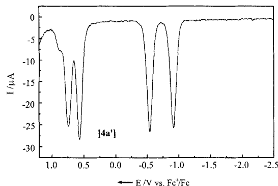
Figure 9. Square-wave voltammogram of 4a' in \text{CH}_3\text{CN} (0.10 M [\text{N}(\text{nBu})_4]\text{PF}_6 ); other conditions as in Figure 7.
