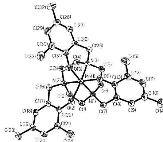
Figure 5. Structure of the neutral complex 4b .
