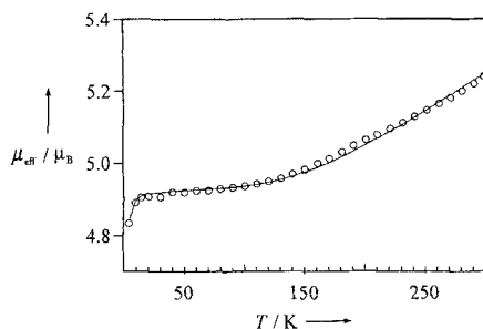
Figure 15. Temperature dependence of the magnetic moment, \mu_{\text{eff}}/\mu_B , of [3a]\text{ClO}_4 . The solid line represents a best fit to the spin Hamiltonian H = -2JS_1 \cdot S_2 ( S_1 = 5/2 ; S_2 = 1/2 ) (see text).
