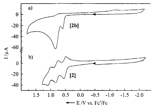
Figure 6. Cyclic voltammograms of 2b (top) and 2 (bottom) in \text{CH}_3\text{CN} (0.10 M [\text{N}(\text{nBu})_4]\text{PF}_6 at a glassy carbon electrode; scan rate: 200 \text{ mVs}^{-1} ; [complex] \approx 10^{-3} M; 298 K).
