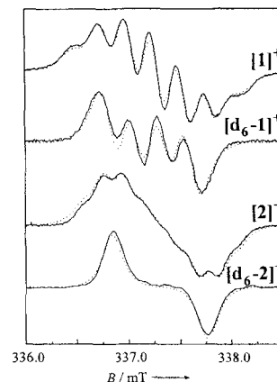
Figure 16. X-band EPR spectra of electrochemically generated [1]^+ , [\text{D}_6\text{-}1]^+ , [2]^+ and [\text{D}_6\text{-}2]^+ in \text{CH}_3\text{CN} (0.10 M [\text{N}(\text{nBu})_4]\text{PF}_6 ) at 298 K (conditions: 9.4592 GHz, 0.45 mW; modulation frequency: 100 kHz; modulation amplitude: 0.026 mT). Solid lines represent experimental spectra, broken lines are simulations using the parameters in Table 5. The ordinates are in arbitrary units of \text{dX}/\text{dB} .
