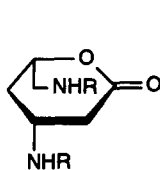
3: R= H 4: R= Ac
