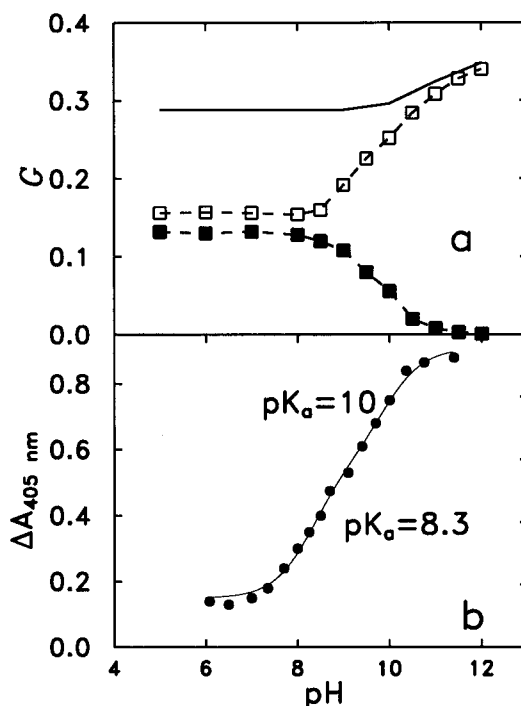
Figure 6. (a) Variation of G(NH_3) (■) and G(I^-) (□) with pH for e_{aq}^- reaction. G(e_{aq}^-) shown for comparison (—). (b) Transient absorption ( \Delta A \times 100 ) at 405 nm in the similar matrix vs the pH.
