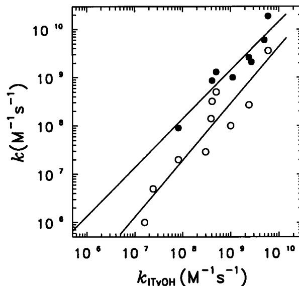
Figure 4. Comparison of bimolecular rate constants for oxidation of ITyOH/ITyO• with secondary oxidizing radicals and •O - against bimolecular rate constants for oxidation of tyrosine (○) and 3,5-diiodotyrosine (●).
