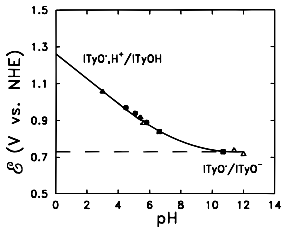
Figure 5. Plot of measured one-electron reduction potential ( E ) vs matrix pH. Reference couples: (▲) I_2^-/2I^- ; (●) NO_2^-/NO_2^- ; (■) CyS^-/CyS^- , and (△) SO_3^-/SO_3^{2-} . Absorbed dose 5 Gy in each case. Solid line represents the variation of E taking into account the pK_a of 8.3 of the phenolic group. From plots E^0 = 0.73 V for ITyO^\bullet/ITyO^- and 1.26 V for ITyO^\bullet, H^+/ITyOH couples.
