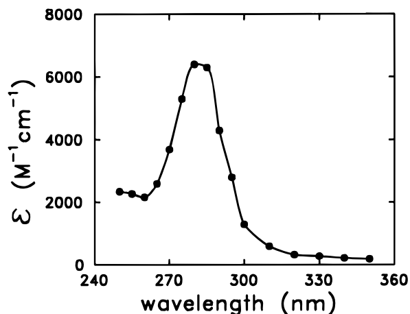
Figure 7. Absorption spectrum of \cdot\text{TyOH} transient at pH 7, 6 \mu\text{s} after pulse; absorbed dose 10 Gy. Matrix: 0.1 M t -BuOH, \text{N}_2 saturated, [\text{ITyOH}] = 0.8 \text{ mM} .
