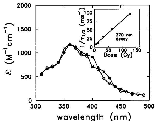
Figure 9. Absorption spectrum of \text{ITyOH}_2^* transient 8 \mu\text{s} after pulse; (●) pH 1.5 with \text{HClO}_4 and (○) pH 5 with 1 M \text{KH}_2\text{PO}_4 , absorbed dose 20 Gy. Matrix: 0.2 M t -BuOH, \text{N}_2 saturated, [\text{ITyOH}] = 0.8 \text{ mM} . Inset: variation of (1/\tau_{1/2})_{\text{first}} for \text{ITyOH}_2^* decay vs [\text{ITyOH}_2^*]_{\text{max}} (proportional to the absorbed dose).
