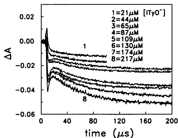
Figure 8. Bleaching signal observed at 310 nm at pH 12 with increasing [\text{ITyO}^-] in the matrix (10 mM phosphate buffer, \text{N}_2 saturated, 0.1 M t -BuOH, and absorbed dose = 50 Gy; G(\text{e}_{\text{aq}}^-) = 0.34 ).
