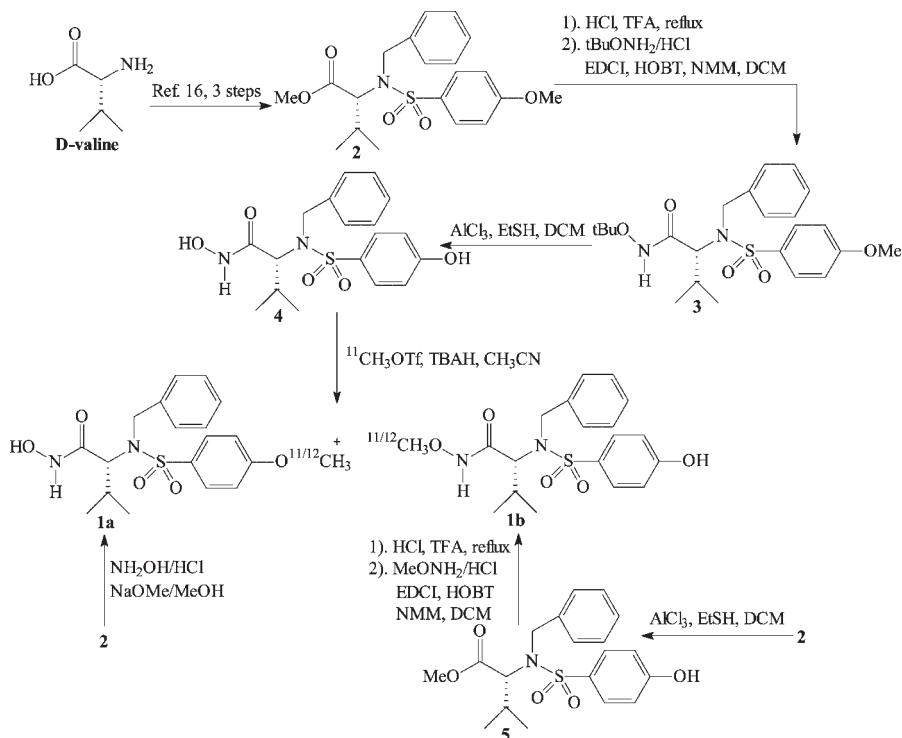
Scheme 1. Synthesis of [ ^{11/12}\text{C} ]CGS 25966 and [ ^{11/12}\text{C} ]CGS 25966 Isomer
