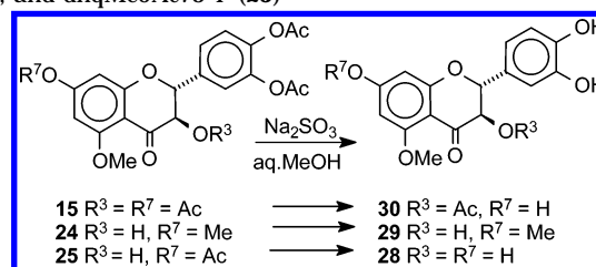
Scheme 3. Deacetylation of dhqMe5Ac373'4' ( 15 ), dhq57Ac3'4' ( 24 ), and dhqMe5Ac73'4' ( 25 )
