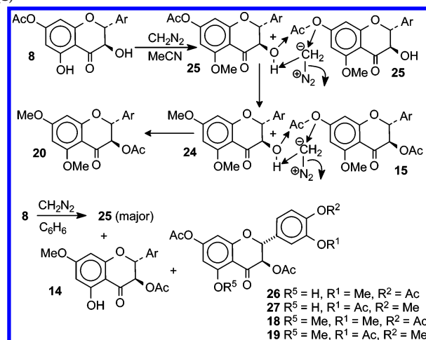
Scheme 2. Methylation of Dihydroquercetin 7,3',4'-triacetate ( 8 ) a
