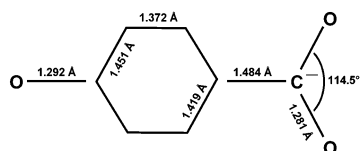
Figure 1. UB3PW91 structure of ^-\text{O}_2\text{C}-\text{PhO}^* (see text).
