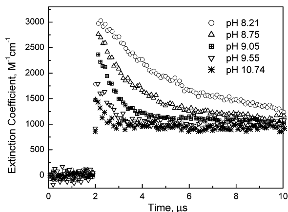
Figure 9. Time dependence of the 365 nm absorption at pH 8.21, 8.75, 9.05, 9.55, and 10.74 for \text{N}_2\text{O} -saturated aqueous solution of 10 mM ^-\text{O}_2\text{C-PhOH} with 5 mM phosphate buffer.
