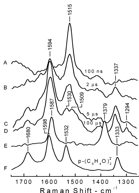
Figure 4. 435 nm Raman spectra observed on electron pulse irradiation of a \text{N}_2\text{O} -saturated aqueous solution containing 5 mM ^-\text{O}_2\text{C-PhOH} and 0.1 M \text{NaN}_3 at pH 11. Time-interval (A) 100 ns, (B) 2 \mu\text{s} , (C) 5 \mu\text{s} , and (D) 100 \mu\text{s} . (E) No electron beam. Spectra in A–D are depicted after subtraction of (E) from the raw spectra. (F) Spectrum of the p,p' -biphenylsemiquinone anion radical, (\text{OPh-PhO})^{\cdot-} , at pH 11.
