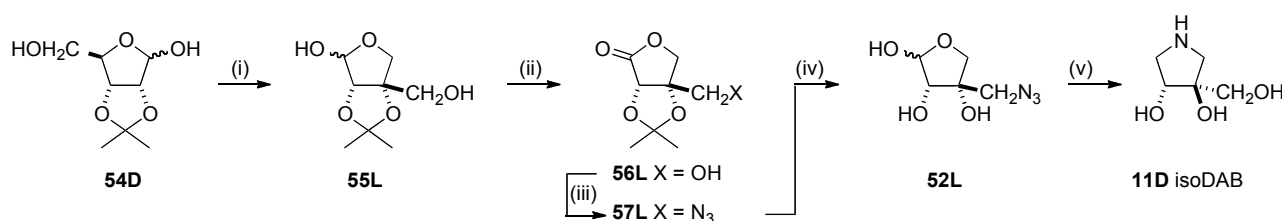
Scheme 6: Reagents and conditions: (i) CH 2 O, K 2 CO 3 , MeOH, H 2 O, reflux, 6 h; then NaBH 4 , H 2 O, rt, 1.33 h; then NaIO 4 , H 2 O, rt, 1 h, 84% (from 54D ) (ii) Br 2 , BaCO 3 , H 2 O, 0 °C to rt, 3 h, 90% (iii) (CF 3 SO 2 ) 2 O, pyridine, CH 2 Cl 2 , -30 °C, 1 h; then NaN 3 , DMF, rt, 24 h, 67% (iv) DIBALH, CH 2 Cl 2 , -78 °C, 1 h, 93% (v) Dowex (50W-X8 H + form) H 2 O:1,4-dioxane, 4:1, 75 °C, 18 h; then Pd/C (10%), H 2 , H 2 O:AcOH, 9:1, 24 h, 71%.
