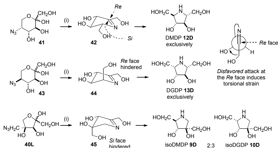
Scheme 4: Diastereoselectivity in the hydrogenation of azidoketoses. Reagents: (i) \text{H}_2 , Pd/C, \text{H}_2\text{O} .
