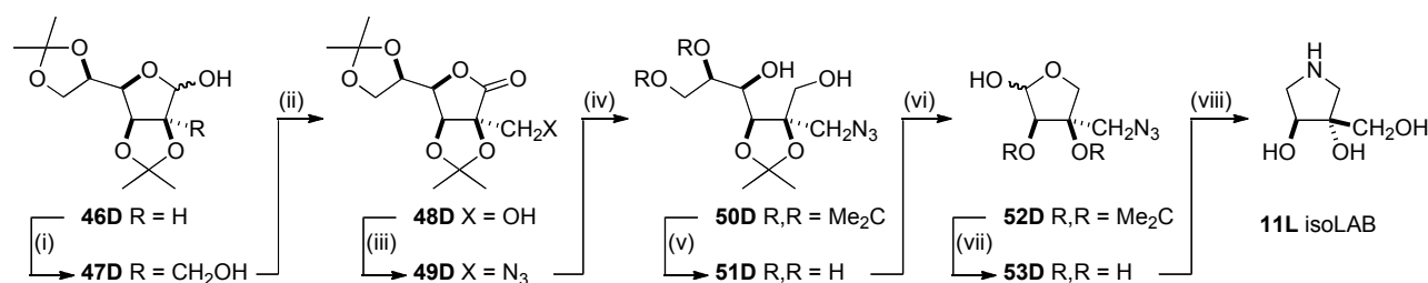
Scheme 5: Reagents and conditions: (i) \text{CH}_2\text{O} , \text{K}_2\text{CO}_3 , MeOH, \text{H}_2\text{O} , reflux, 5 h, 74% (ii) \text{Br}_2 , \text{BaCO}_3 , \text{H}_2\text{O} , 0 °C to rt, 32 h, 80%, or \text{I}_2 , \text{K}_2\text{CO}_3 , ^t\text{BuOH} , 100 °C, 81% (iii) (\text{CF}_3\text{SO}_2)_2\text{O} , pyridine, \text{CH}_2\text{Cl}_2 , -30 °C; 2.5 h then \text{NaN}_3 , DMF, rt, 3 h, 96% (iv) DIBALH, \text{CH}_2\text{Cl}_2 , -78 °C, 2 h; then \text{NaBH}_4 , MeOH, 0 °C to rt, 2.5 h, 68% (v) \text{H}_2\text{O}:\text{AcOH} , 1:1, rt, 16 h, 78% (vi) \text{NaIO}_4 , \text{H}_2\text{O} , rt, 18 h, 85% (vii) Dowex (50W-X8 \text{H}^+ form) \text{H}_2\text{O}:\text{1,4-dioxane} , 4:1, 60 °C, 36 h, 91% (viii) Pd/C (10%), \text{H}_2 , \text{H}_2\text{O}:\text{AcOH} , 9:1, rt, 24 h, 81%.
