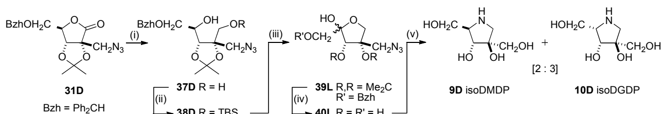
Scheme 3: Reagents and conditions: (i) NaBH 4 , EtOH: t BuOH 13:2, rt, 1.5 h, 97%; (ii) t -BuMe 2 SiCl, imidazole, DMF, 0 °C, 5 h, 98%; (iii) Dess-Martin periodinane, CH 2 Cl 2 , rt, 2 h; then TBAF, THF, 0 °C to rt, 2 h, 92%; (iv) p TsOH, H 2 O, 1,4-dioxane, 85 °C, 18 h, 63%; (v) H 2 , Pd (10% on C), H 2 O, rt, 18 h, 83%.
