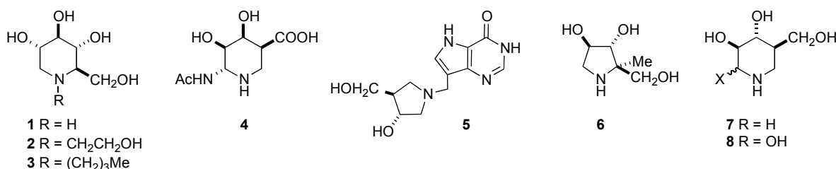
Figure 1: Structures of iminosugars
