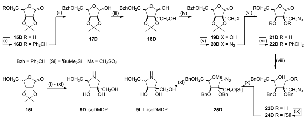
Scheme 1: Reagents and conditions: (i) Ph 2 CN 2 , PhMe, reflux, 2 h, 92%; (ii) DIBALH, CH 2 Cl 2 , -78 °C, 1 h, 99%; (iii) CH 2 O, K 2 CO 3 , MeOH, H 2 O, reflux, 4 h, 74%; (iv) I 2 , K 2 CO 3 , t -BuOH, reflux, 1 h, 85%; (v) (CF 3 SO 2 ) 2 O, pyridine, CH 2 Cl 2 , -30 °C, 1 h; then NaN 3 , DMF, rt, 18 h, 100%; (vi) AcCl, MeOH, reflux, 18 h, 97%; (vii) BnBr, NaH, DMF, 0 °C, 4.5 h, 86%; (viii) NaBH 4 , EtOH, rt, 3 h, 100%; (ix) t -BuMe 2 SiCl, imidazole, DMF, 0 °C to rt, 6 h, 94%; (x) MsCl, Et 3 N, CH 2 Cl 2 , 0 °C to rt, 2 h, 99%; (xi) H 2 , Pd (10% on C), NaOAc, H 2 O, 1,4-dioxane, rt, 24 h; then H 2 , Pd (10% on C), HCl, H 2 O, 1,4-dioxane, rt, 48 h, 100%.
