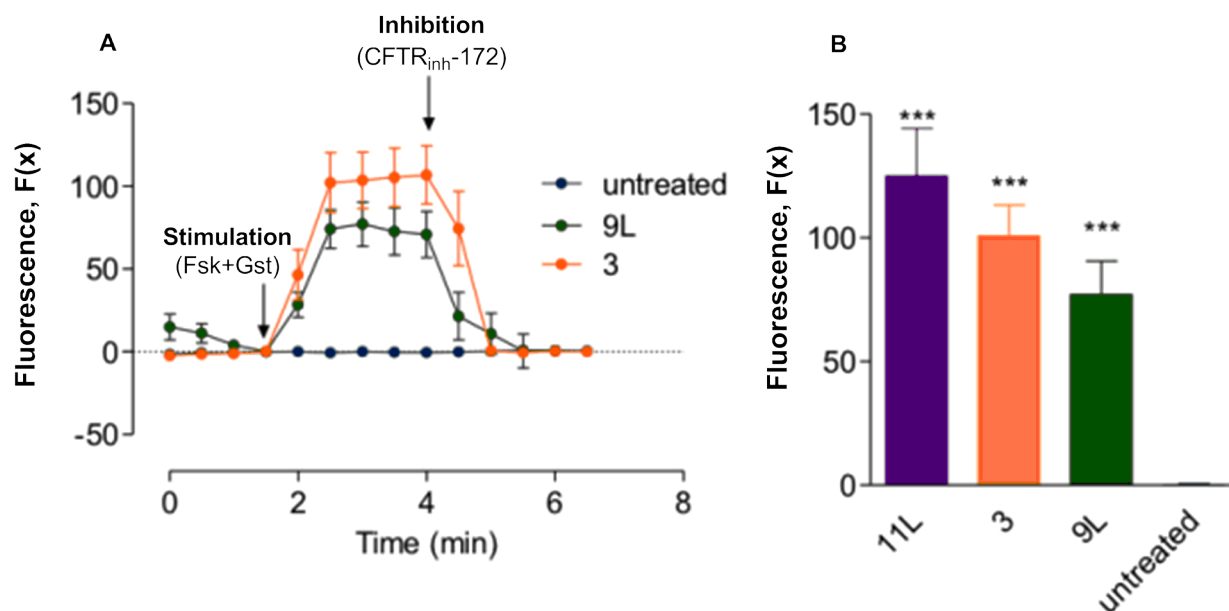
Figure 4: Effect of L-isoDMDP 9L , isoLAB 11L and Miglustat 3 on the activity of F508del-CFTR assessed by single-cell fluorescence imaging using the potential-sensitive fluorescent probe bis-(1,3-diethylthiobarbituric acid) trimethine oxonol, and its sensitivity to the CFTR selective inhibitor CFTR inh -172 using the human airway epithelial CF-KM4 cell line.
