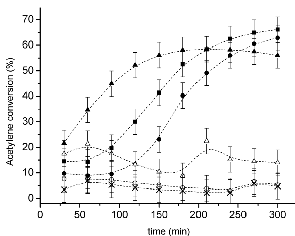
Fig. 1 Acetylene conversion over Au/C (1 wt%) catalysts subject to reduction and oxidation cycles, (■) fresh catalyst, (○) reduced catalyst, (●) first catalyst oxidation, (Δ) second catalyst reduction, (▲) second catalyst oxidation, (×) third catalyst reduction.
