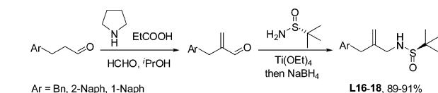
Scheme 2. Synthesis of Optimal Ligands L16 – L18
