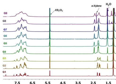
Figure 1. 300 MHz 1 H NMR spectra of G1 and G2 and 500 MHz 1 H NMR spectra of G3–G9 in CD 2 Cl 2 at 298 K.
