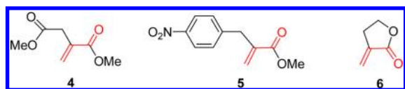
Chart 3. Cyclizing Reagents 4–6
