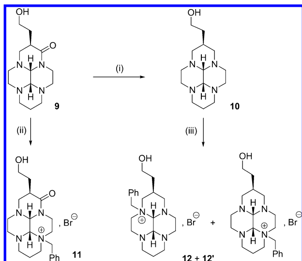
Scheme 2 a
