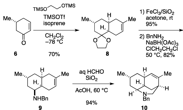
Scheme 2. Diels–Alder Reaction and Aza-Prins Reaction
