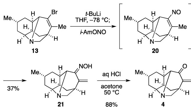
Scheme 6. Transformation into Enone 4 through an Oxime
