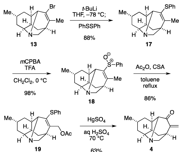
Scheme 5. Transformation into Enone 4 via Vinylogous Pummerer Rearrangement
