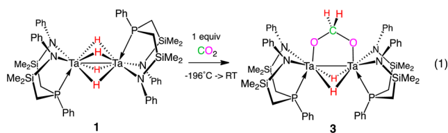
Figure 1. Selected bond lengths (Å) and bond angles (deg) for 3: Ta1–N1 2.091(7), Ta1–N2 2.062(6), Ta1–P1 2.628(2), Ta1–O1 1.980(5), Ta1–Ta1 2.7688(7), N1–Si1 1.742(7), N2–Si2 1.739(7), C1–O1 1.384(7); O1–C1–O1' 117.0(9), Ta1–O1–C1 126.4(5), O1–Ta1–O1' 117.0(9), O1–Ta1–N1 91.6(2), O1–Ta1–N2 91.6(2), N1–Ta1–N2 118.2(3), O1–Ta1–P1 160.99(15), N1–Ta1–P1 77.82(19), N2–Ta1–P1 79.08(19), O1–Ta1–Ta1' 83.45(14).
