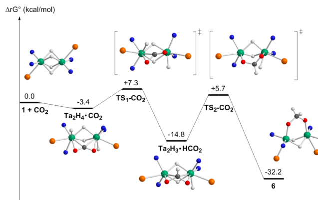
Figure 2. Gibbs free-energy profile of the reaction between the tetrahydride complex 1 and CO 2 . NPN ligands have been simplified for clarity. Atoms colors: Ta, green; P, orange; N, blue; O, red; C, black; H, white. For atom numbering, Ta1 is on the left, while Ta2 is on the right.
