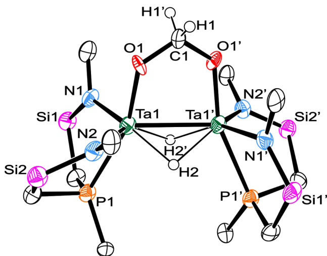
Figure 1. Selected bond lengths (Å) and bond angles (deg) for 3: Ta1–N1 2.091(7), Ta1–N2 2.062(6), Ta1–P1 2.628(2), Ta1–O1 1.980(5), Ta1–Ta1 2.7688(7), N1–Si1 1.742(7), N2–Si2 1.739(7), C1–O1 1.384(7); O1–C1–O1' 117.0(9), Ta1–O1–C1 126.4(5), O1–Ta1–O1' 117.0(9), O1–Ta1–N1 91.6(2), O1–Ta1–N2 91.6(2), N1–Ta1–N2 118.2(3), O1–Ta1–P1 160.99(15), N1–Ta1–P1 77.82(19), N2–Ta1–P1 79.08(19), O1–Ta1–Ta1' 83.45(14).
