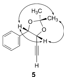
Fig. 2. NOESY Correlations (H \leftrightarrow H) of 5
