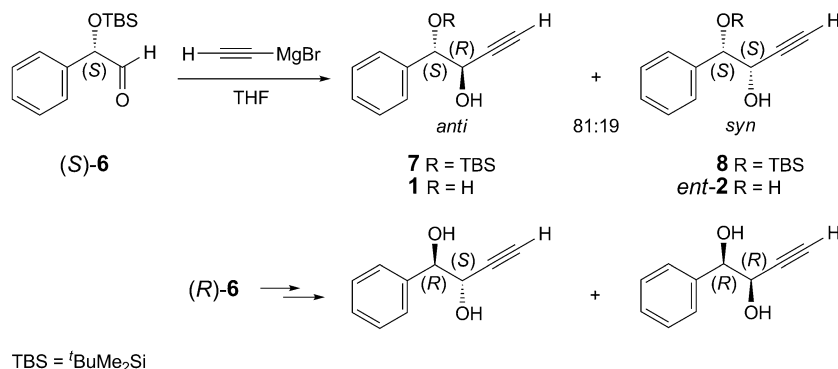
Scheme. Synthesis of 1 and 2 , and Their Enantiomers
